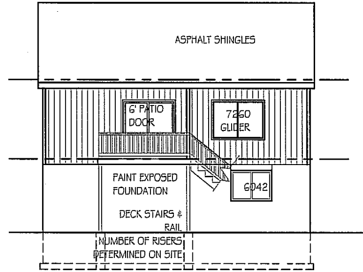
REAR ELEVATION
