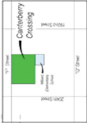
VICINITY MAP
